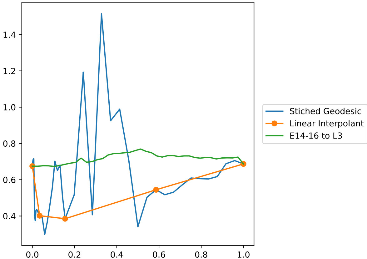
Average Ricci Curvature
